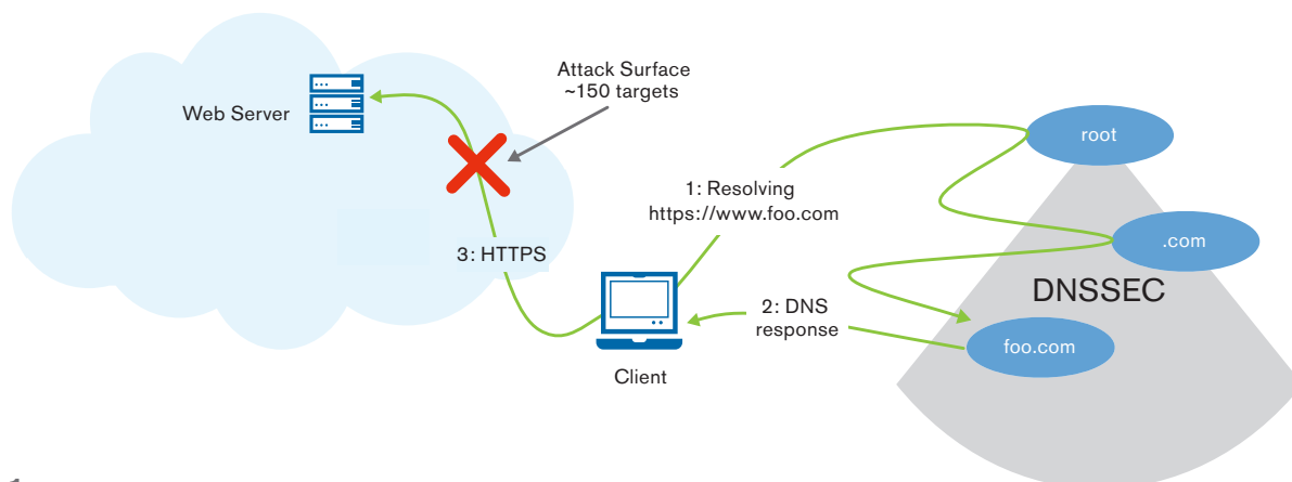
FIGURE 1: THE VULNERABILITY OF AN HTTP SESSION
