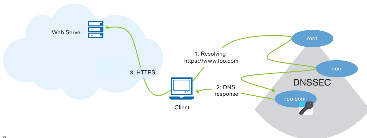
FIGURE 6: ATTACK SURFACE OF DANE
