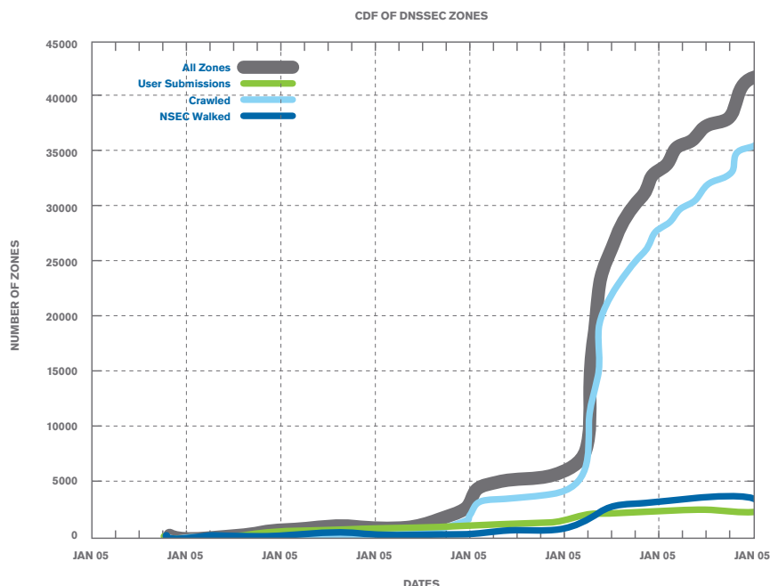
FIGURE 3: THE SIZE OF THE GLOBAL GROWTH OF DNSSEC, AS SEEN BY SECSPIDER
