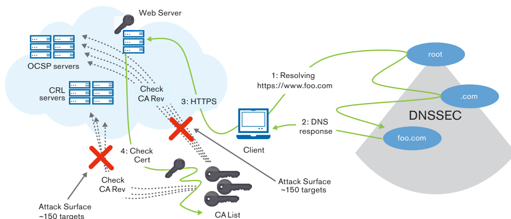
FIGURE 2: ATTACK SURFACE USING CAs
