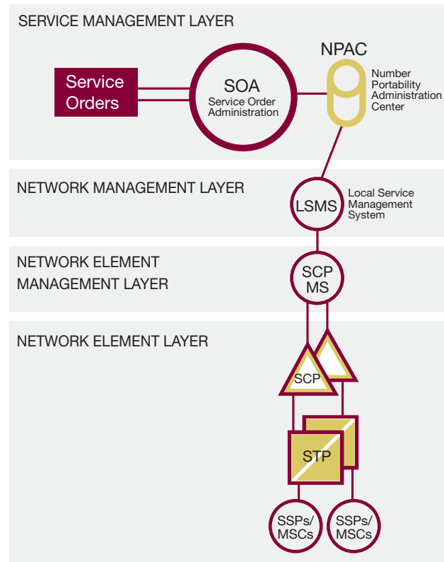
Figure 1 LNP ARCHITECTURE
