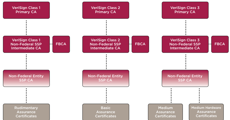
Figure 1: Non-Federal SSP PKI Hierarchy
